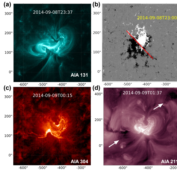
Fig. 5: AR 12158 associated with CME1 eruption in different wavelengths - (a) AIA 131 Å image highlights the evolved sigmoid and the hooks corresponding to flux rope footpoints during the early phase of the flare; (b) HMI magnetogram saturated at \pm 200 G overlaid with the approximated PIL orientation (i.e., the part of the extended PIL that most likely erupted as CME1), before the start of the flare; (c) AIA 304 Å image shows the inverse J-shaped flare ribbons after the eruption, which suggest the eruption of a left-handed flux rope, and (d) AIA 211 Å image shows the post flare coronal dimmings (marked with white arrows). The X - and Y -axes correspond to the helio-projective longitude and latitude, respectively.
