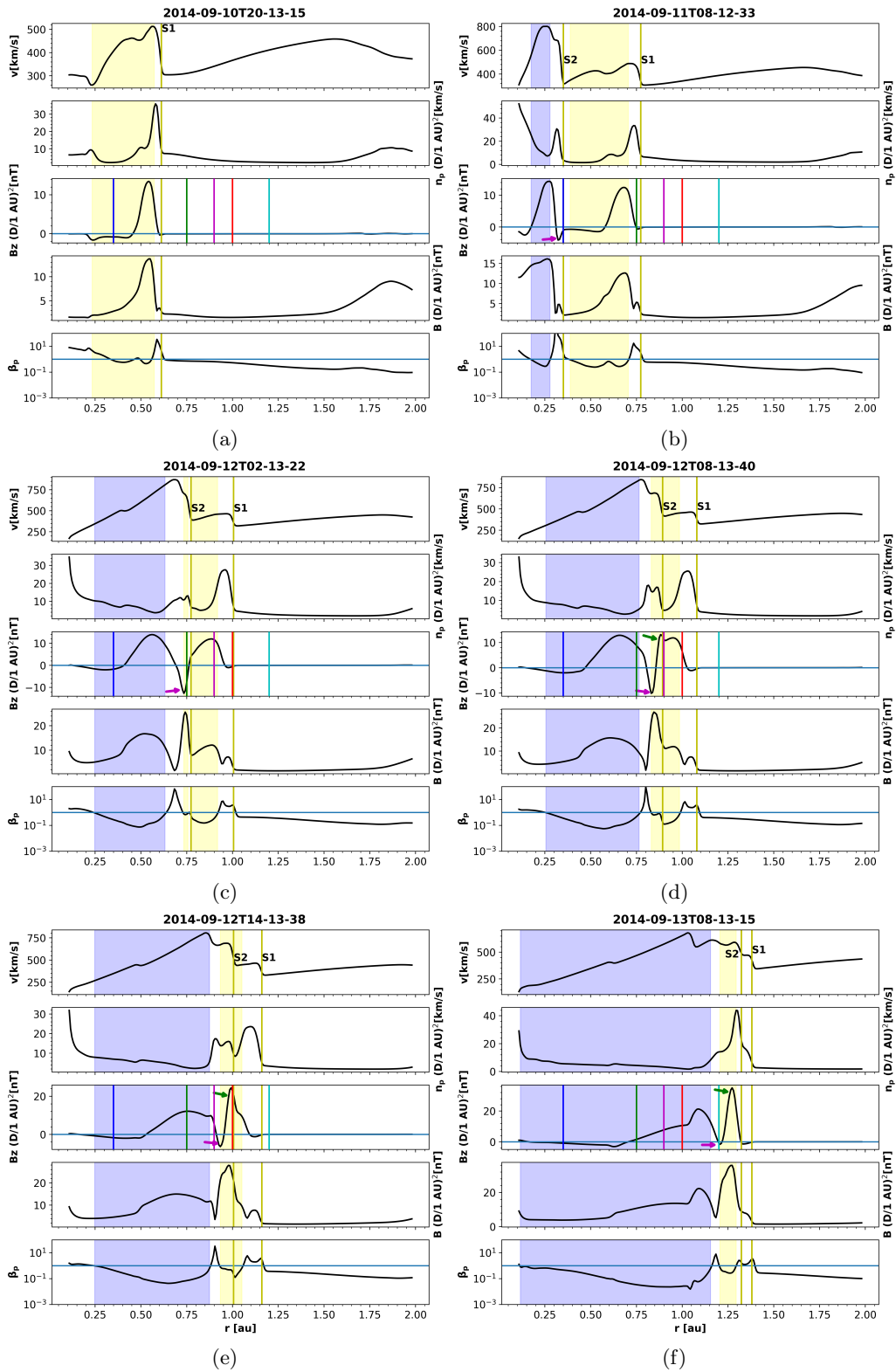
Fig. 13: Radial evolution profile of the CME1 and CME2 along Sun-Earth line at different times of propagation and interaction extracted from Run4. Top to bottom (in each plot): speed ( v ), proton number density ( n_p ), z-component of magnetic field ( B_z ), total magnetic field ( B ), and proton plasma beta ( \beta_p ). The yellow and blue shaded areas depict the extent of magnetic ejecta of CME1 and CME2 respectively extracted using the criterion \beta_p < 1 ( \beta_p < 5 in (a)). All physical quantities except the speed are scaled by (D/1 \text{ au})^2 where D is the radial distance from the Sun. The CME shocks (S1 and S2) are marked in yellow lines. The colourful vertical lines in the B_z panel correspond to different radial distances to explain various phases of Run4 (detailed in Section 6.3): (a) Propagation of CME1 alone in the heliosphere; (b) Formation of a compressed negative B_z ejecta CE1a (shown with magenta arrow); (c) Further compression of CE1a; (d) Development of a compressed positive B_z ejecta, CE1b (shown with green arrow), ahead of CE1a (e) Further compression of CE1b; and (f) Diffusion of CE1a ( \sim 0 nT) upon reaching 1.2 au while CE1b undergoes further enhanced.
