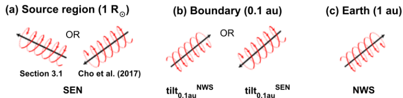
Fig. 8: Schematic representation of the CME2 orientation inferred from different observational proxies at different locations - (a) Close to 1 R_{\odot} , based on the analysis of the source region in Section 3.1 and the analysis of Cho et al. (2017); (b) Close to the 0.1 au, based on the 3D reconstruction of the white-light images (Section 3.3); (c) At 1 au, based on the in situ observations (Section 4).
