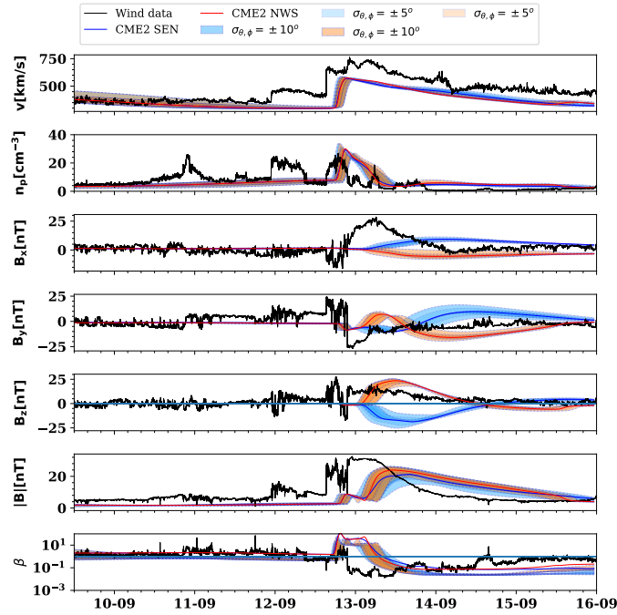
Fig. 10: Time series plot showing the comparison between the simulations with different orientations of CME2 modelled with FRi3D, at Earth - Run1 (blue) is simulated with \text{tilt}_{0.1\text{au}}^{\text{SEN}} (deduced based on the orientation close to 1 R_{\odot} ) and Run2 (red) with \text{tilt}_{0.1\text{au}}^{\text{NWS}} (similar to the tilt at 1 au). Both the orientations follow the same geometrical tilt derived from the 3D reconstruction at 0.1 au but with two different axial magnetic field orientations. From top to bottom: speed ( v ), proton number density ( n_p ), B_x , B_y , B_z , magnetic field strength ( |B| ) and plasma beta ( \beta ). The solid line and the shaded regions show the profile at Earth and in the 5\text{-}10^\circ latitudinal and longitudinal offset around Earth respectively.
