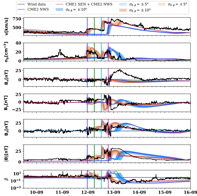
Fig. 12: Results of Run2 (blue; CME2 NWS) and Run4 (red; CME1 SEN + CME2 NWS) are compared. CME1 and CME2 parameters in Run4 correspond to Run3 and Run2 respectively. Figure description is similar to Fig. 10. S1, the start of ME1, S2 and the start of ME2 are marked with blue, green, cyan and magenta vertical lines respectively in Run4.
