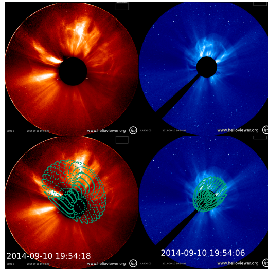
Fig. B.2: Coronagraph images of CME2 development on September 10, 2014 as observed by COR2 (STEREO-B) and C3 (LASCO) (top). The same images overlaid with the 3D reconstruction using the FRi3D model (bottom).
