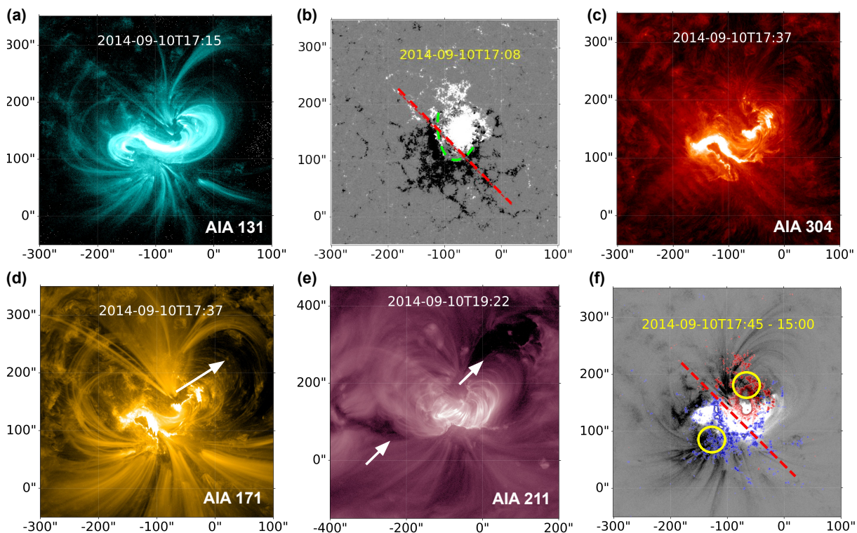
Fig. 6: AR 12158 associated with CME2 eruption in different wavelengths - (a) AIA 131 Å image before CME2 eruption; (b) HMI magnetogram saturated at \pm 200 G overlaid with the approximated PIL drawn with a red dashed line; (c) AIA 304 Å image highlights the inverse J-shaped flare ribbons indicating left-handedness of the flux rope; (d) AIA 171 Å image showing the coronal loops and the eruption direction of CME2 in north-westward direction as per Dudík et al. (2016) ; (e) AIA 211 Å image showing coronal dimmings marked with white arrows; (f) AIA 131 Å base-difference image overlaid with HMI magnetogram contours saturated at \pm 1000 G coloured blue (red) for negative (positive) polarity. The yellow circles demarcate the dimmings located at the footpoints of the FR. The red dashed line is the approximated PIL. The X - and Y -axes correspond to the helio-projective longitude and latitude, respectively.
