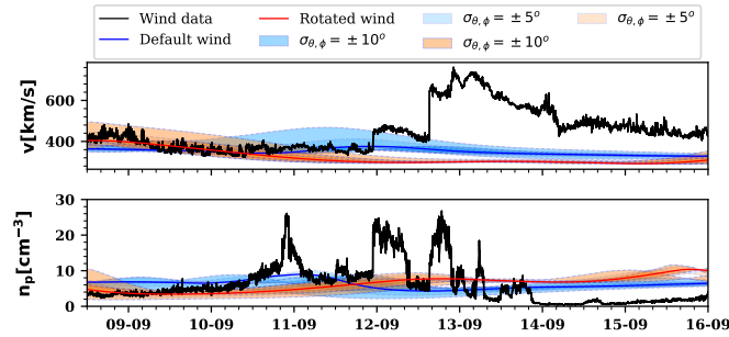
Fig. 9: Background solar wind modelled with the default EUHFORIA coronal model setup using the synoptic magnetogram from GONG on September 8, 2014, at 23:00 (in blue), and the rotated solar wind (in red). The shaded regions provide an error estimate in \pm 5\text{-}10^\circ in latitude ( \sigma_\theta ) and longitude ( \sigma_\phi ) around Earth. Corresponding WIND observations are plotted in black.
