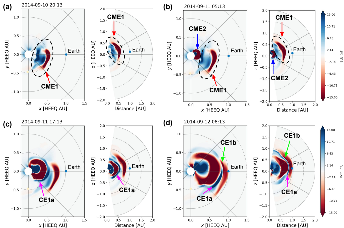
Fig. 14: Evolution of B_z in the heliosphere as simulated in Run4. The co-latitude component in the spherical coordinate system is B_{clt} , which is equivalent to -B_z on the ecliptic plane. The red and blue spectra of the colour bar correspond to positive and negative B_z , respectively. Each sub-figure shows the view of the equatorial (X-Y) and the meridional (X-Z) planes at a particular time mentioned at its top. (a) CME1 in the pre-interaction phase is identified schematically with a dashed ellipse; (b) CME2 is shown evolving behind CME1 in the early stage of interaction; (c) CME2 compressing the interval of the trailing negative B_z component of CME1 to create CE1a (darker blue region) in the sheath ahead of itself; and (d) CE1a is shown to be further compressing the interval of the leading positive B_z component of CME1 to create CE1b (darker red region) during the interaction phase of the event. The animation of this figure can be found in the online version of the paper.
