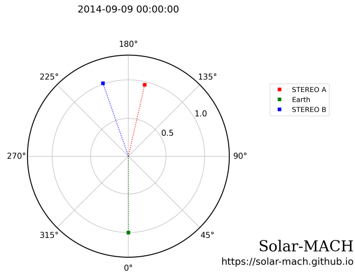
Fig. 2: Position of STEREO-A, STEREO-B and Earth on September 9, 2014, at 00:00. The grid in black corresponds to the Stonyhurst coordinate systems. This polar plot is generated using the Solar-MACH tool ( https://serpentine-h2020.eu/tools/ ; Gieseler et al. 2022).
